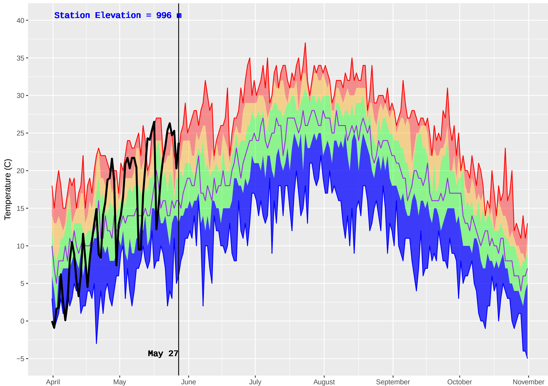
CRANBROOK FS (426) : Historical (2001–2016) and Current (2018) Noon Temperature
