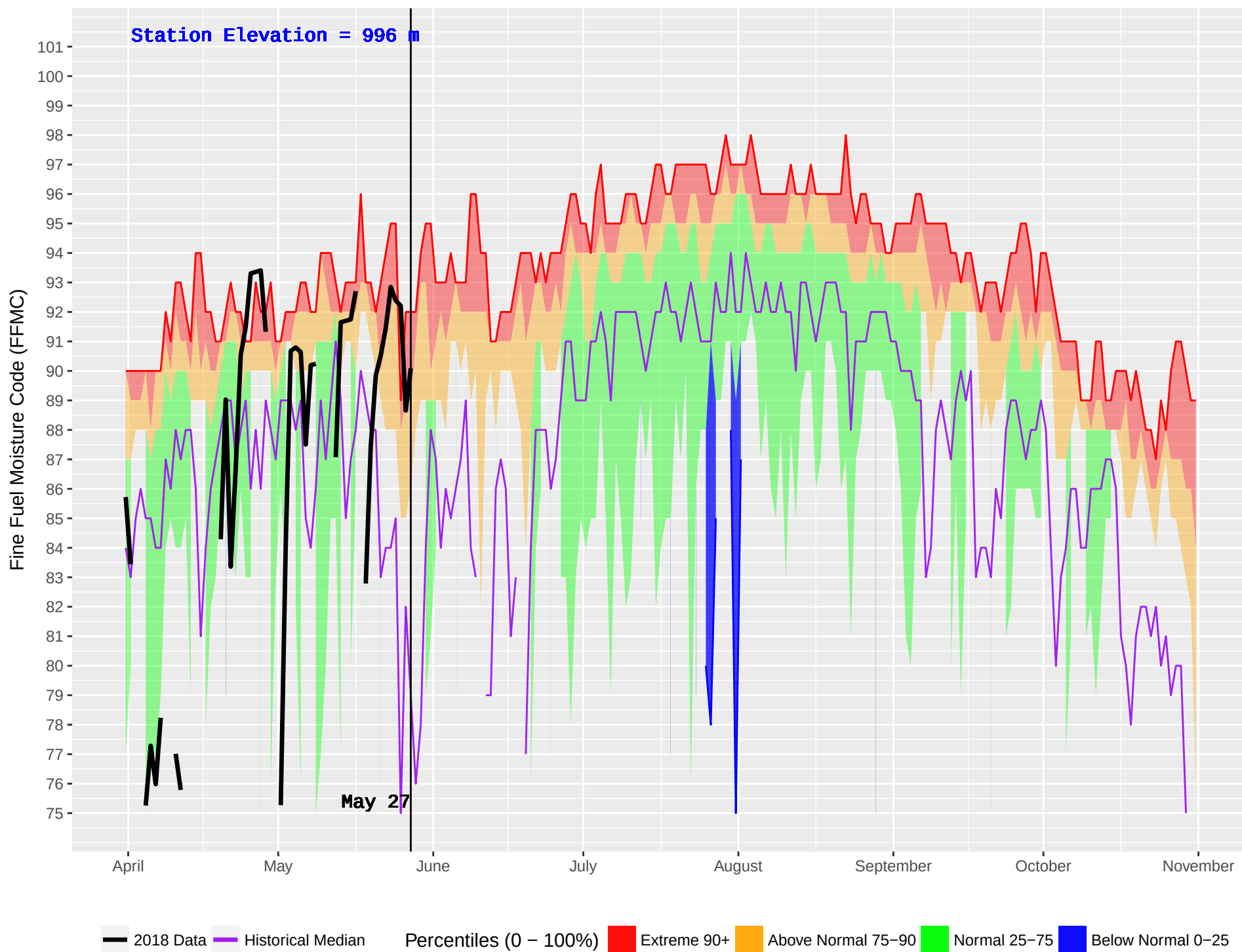
CRANBROOK FS (426) : Historical (2001–2016) and Current (2018) Noon Fine Fuel Moisture Code (FFMC)
